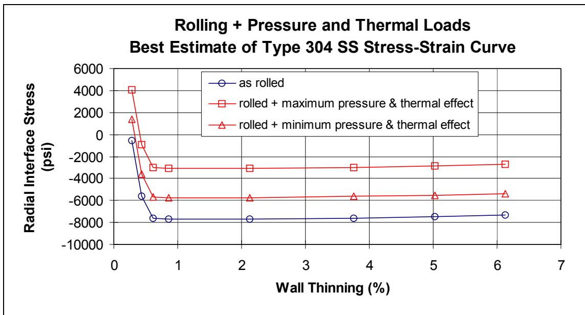
Figure 7 Rolling Repair Induced Radial Interface Stress for As-rolled and for Bounding Operating Conditions
